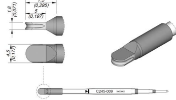
CARTRIDGES TO SOLDER QFP PACKAGE
