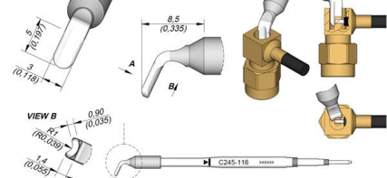
VIEW A
